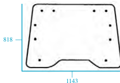
23/4004-5 (D9030, 82004391) Parabrisas abatible - 10 agujeros - claro Windscreen (Opening) - 10 holes - clear
