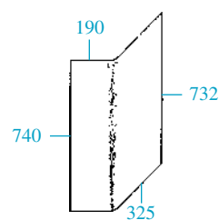
23/4086-3 (5154093) Panel trasero (drcha.) - verde Rear quarter RH - green
