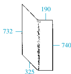
23/4085-3 (5154092) Panel trasero (izq.) - verde Rear quarter LH - green
