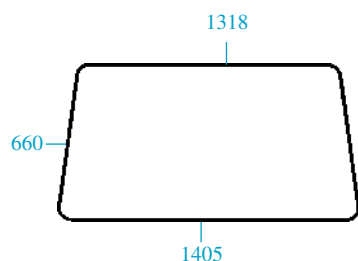
23/4000-47 (D9001, 5113401) Parabrisas Windscreen
