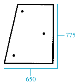
23/4047-66 (D6721, 83995321, 82009812) Lateral drcha. - 3 agujeros Side RH - 3 holes
