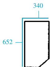
23/4011-13 (D6713, 82001923) Frontal (inf. izq.) - claro Front (Lower LH) - not tinted
