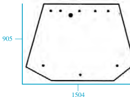
23/4072-31A (D6722/A, 82005316, 5178304) Trasero (superior) - 6 agujeros Upper rear - 9 holes
