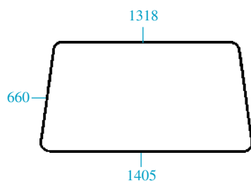
23/4000-47 (D9001, 5113401) Parabrisas Windscreen
