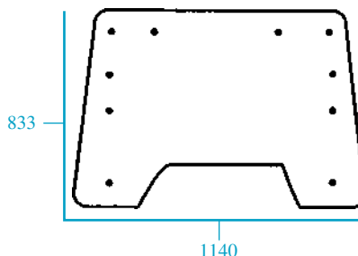
23/4004-4 (D9031, 82000488) Parabrisas abatible - 10 agujeros Windscreen (Opening) - 10 holes
