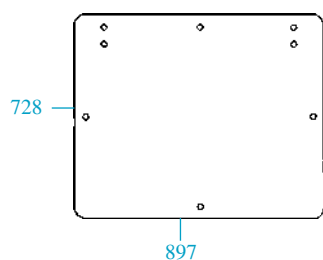
23/4072-84 (5154756) Trasero (superior) 8 agujeros - verde Upper rear - 8 holes - green
