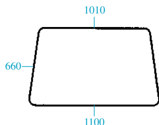
23/4000-46 (D9000, 5108663) Parabrisas Windscreen
