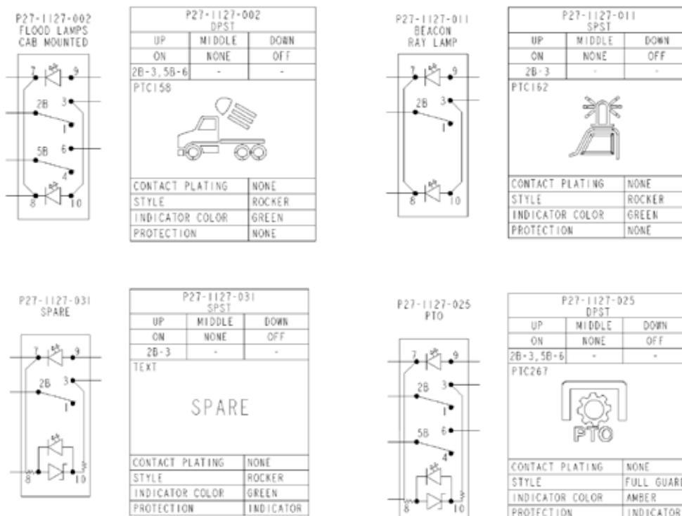
FIGURE 8-15. Optional Switches.
