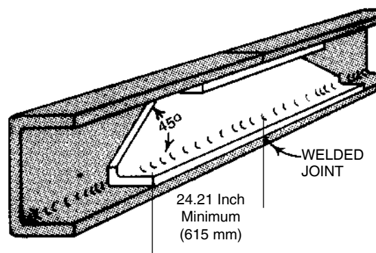
FIGURE 7-2. Frame Insert
