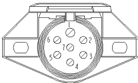
FIGURE 8-32: SAE J560 Trailer Connector
