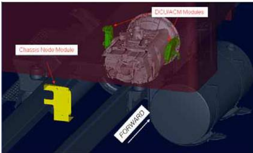
FIGURE 8-27. Aerocab Standard Hardware Locations
