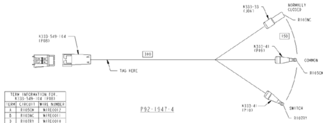
FIGURE 8-17. Spare Relay Harnesses
