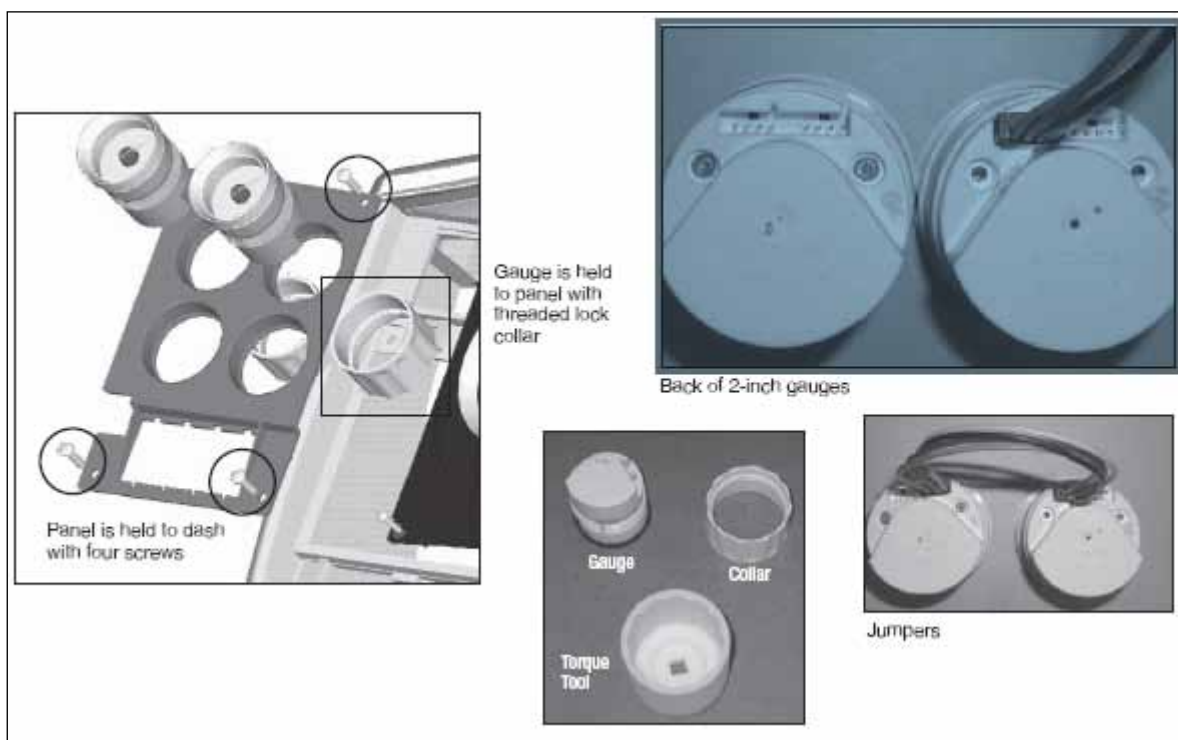
FIGURE 8-6. CVSG Gauges
