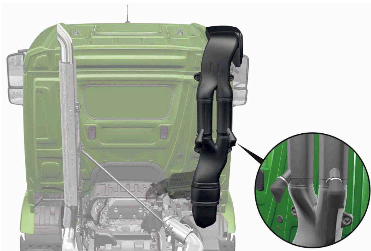
Cyclone prefilter for coarse dust (M8L)
