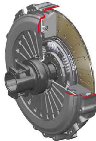
Single-plate clutch
