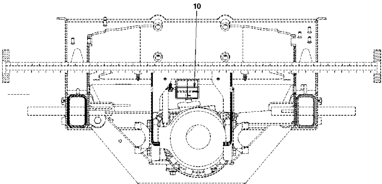
SECTION G-G
