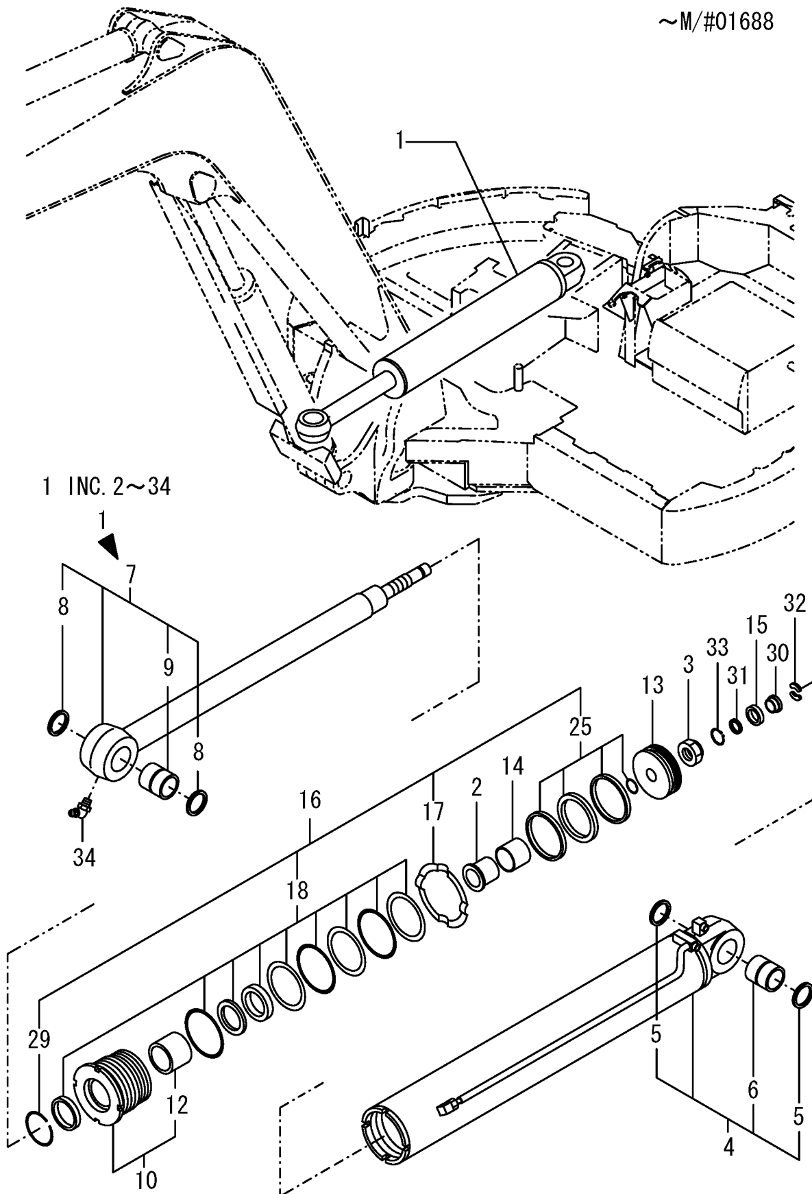
Fig. 73 SWING CYLINDER (NEW)
