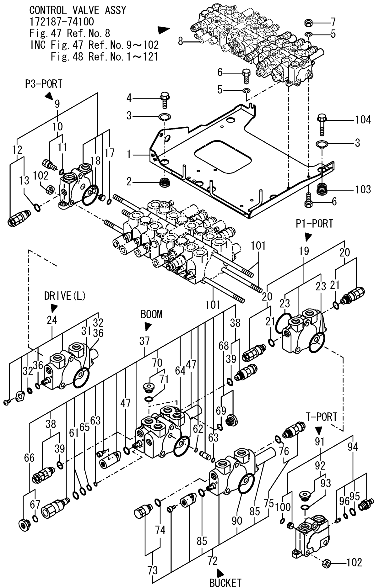
Fig. 47 CONTROL VALVE (1/2)
