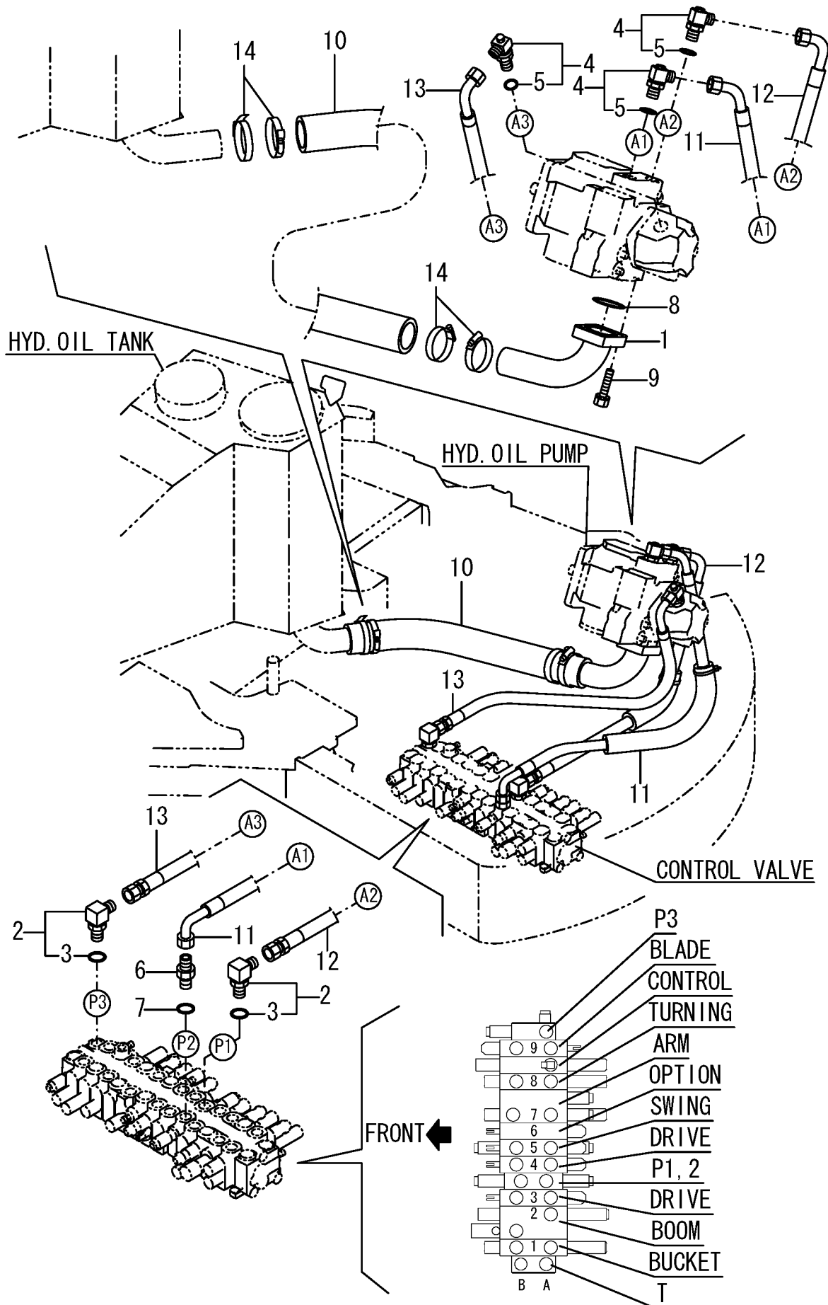
Fig. 53 HYD. OIL PIPING (TANK~PUMP ~VALVE)
