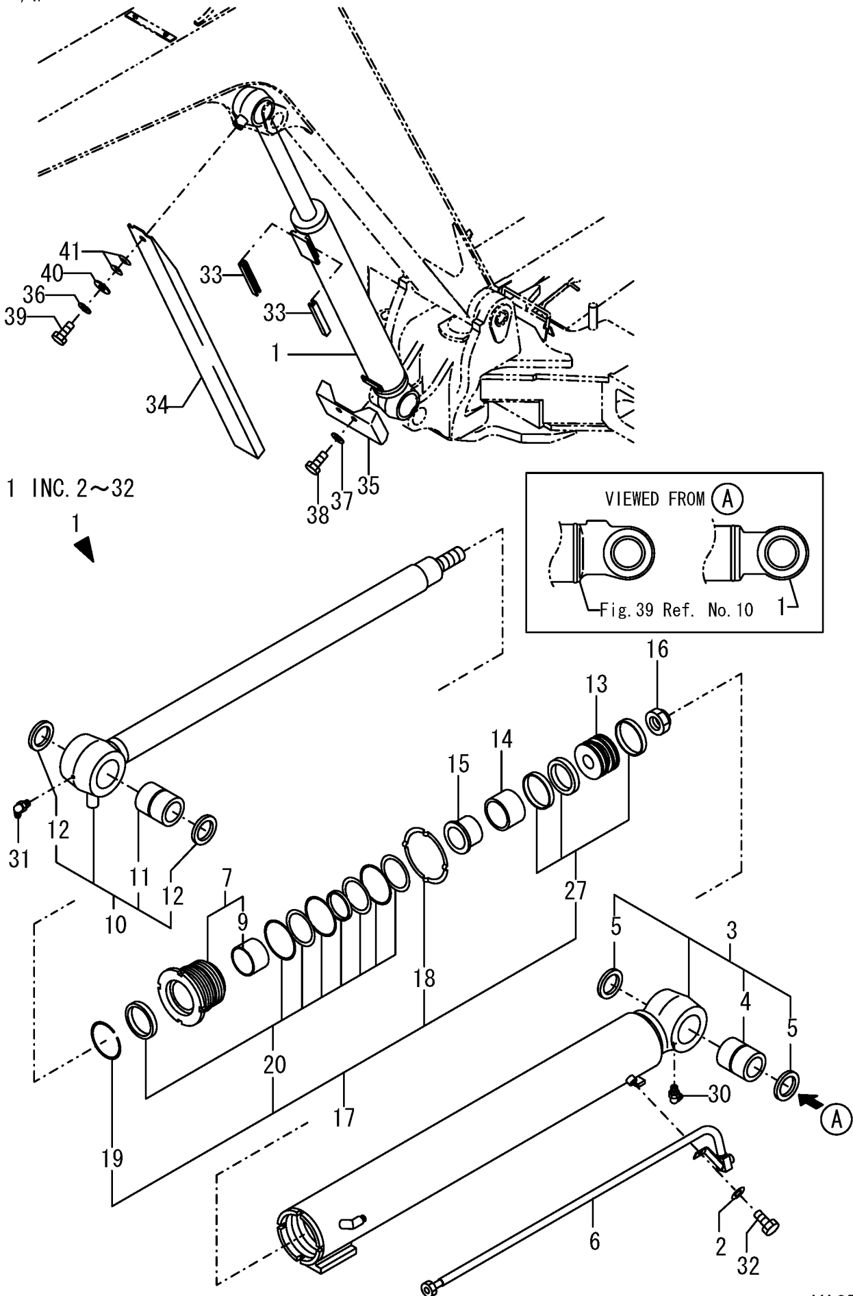
Fig. 70 BOOM CYLINDER (NEW)
