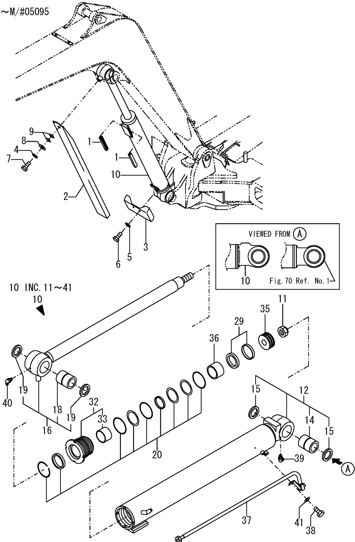
Fig. 39 BOOM CYLINDER (PREVIOUS)
