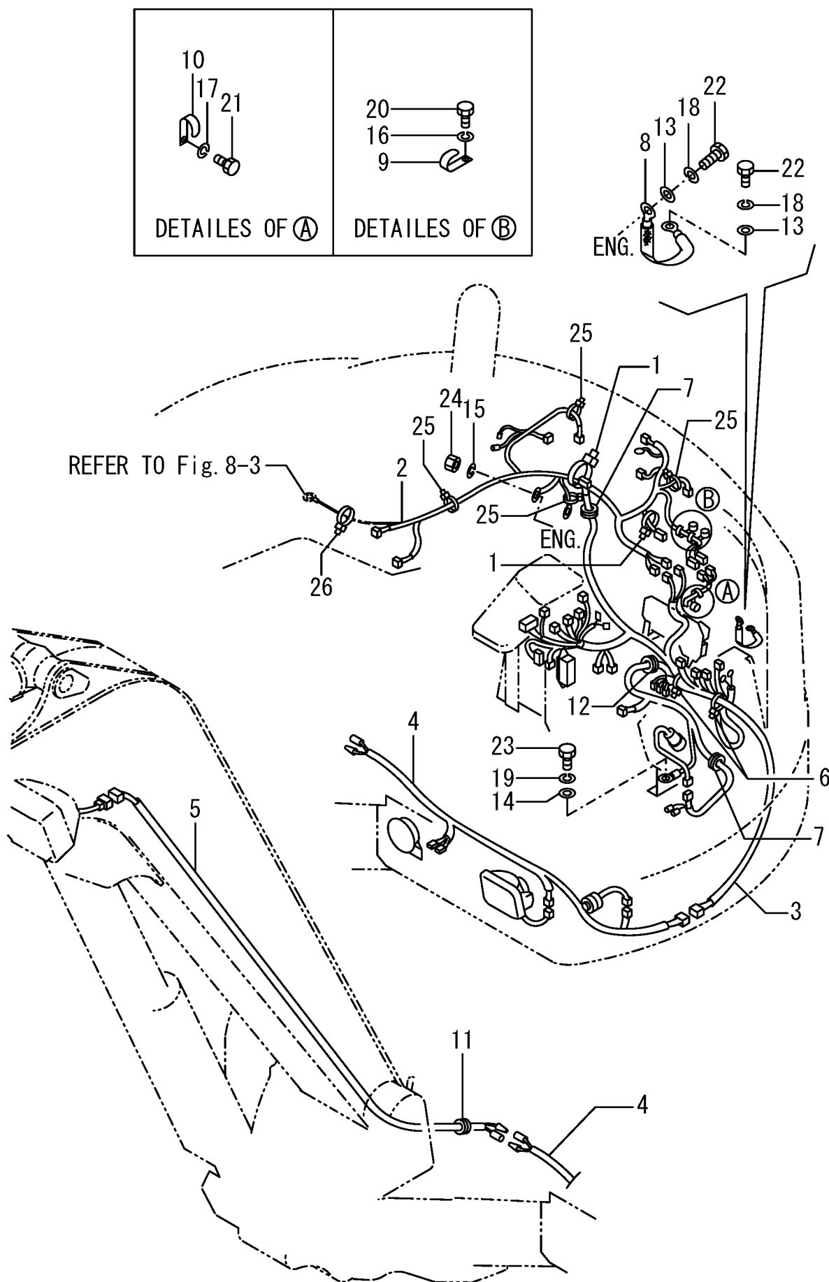
Fig. 9 ELECTRIC PART (WIRING)
