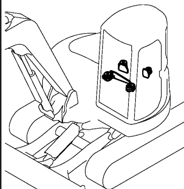
Fig.6 RADIATOR & MOUNT
