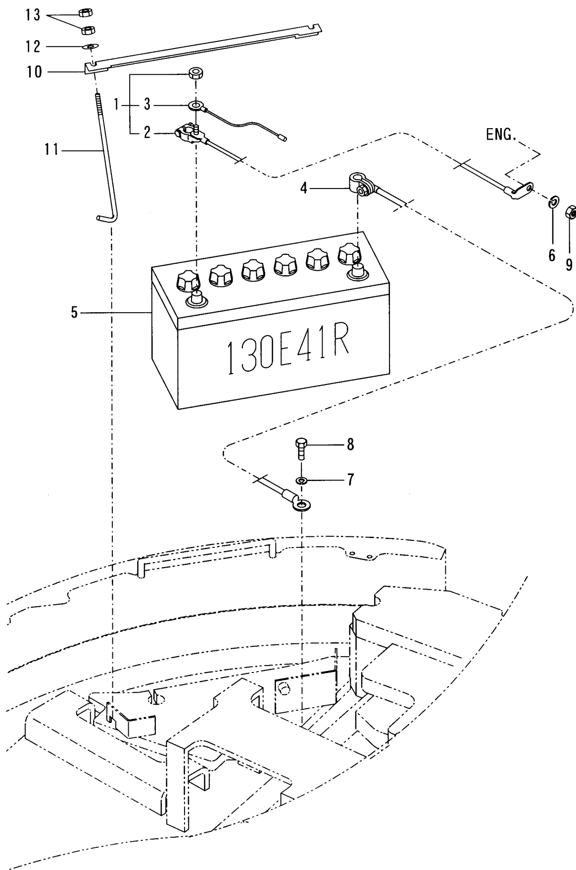
Fig. 8 BATTERY
