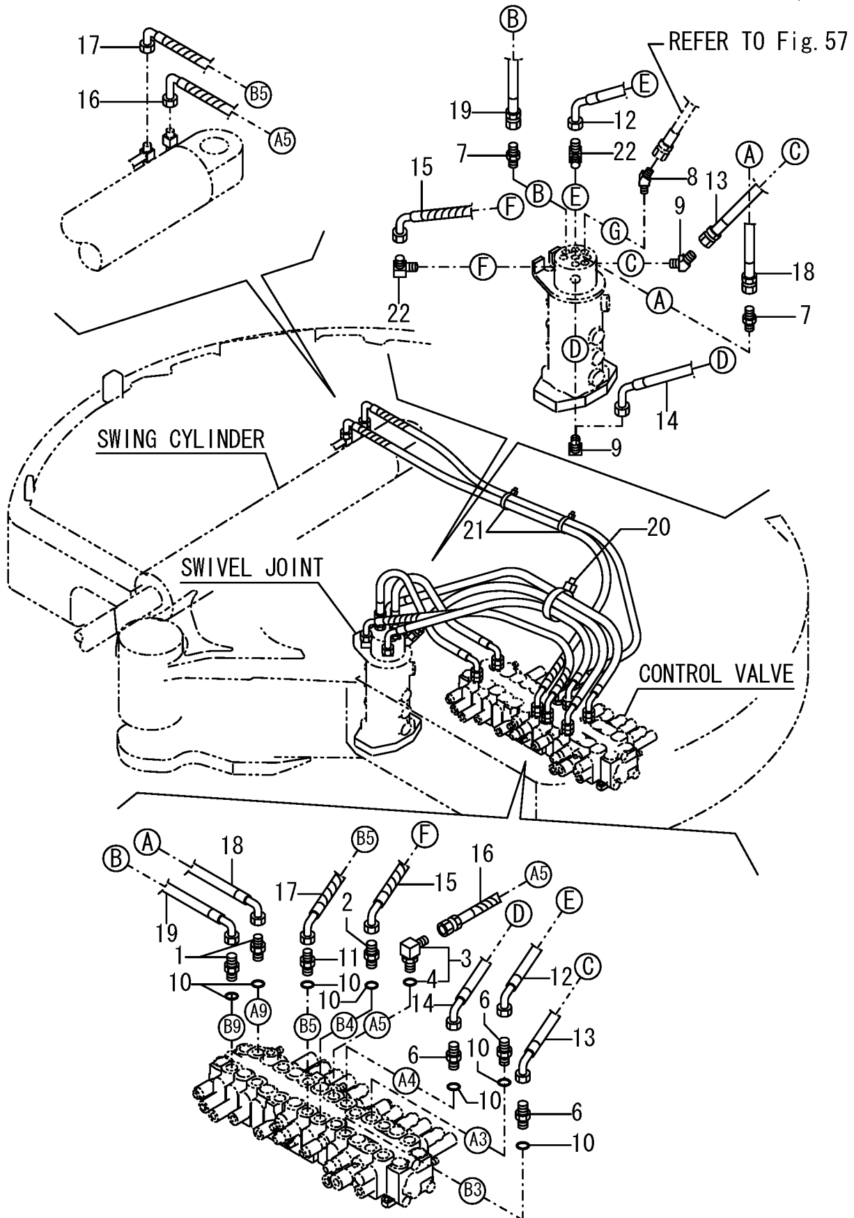
Fig. 55 HYD. OIL PIPING (VALVE~SWIVEL, SWING)
