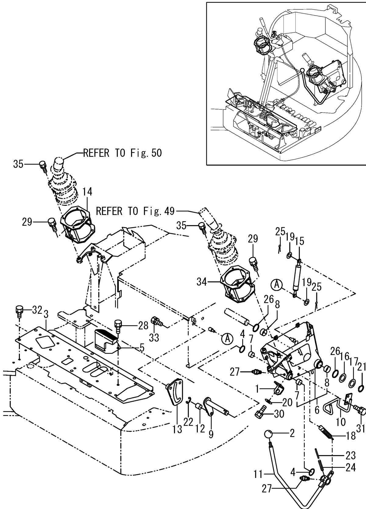
Fig. 18 CONTROL EQUIP. (LEVER STAND & LOCK LEVER)
