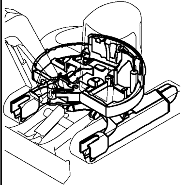
Fig. 24 FRAME & TURNING BEARING
