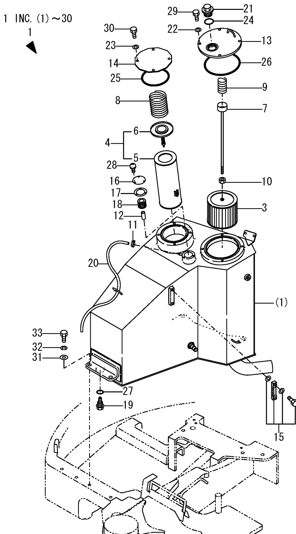
Fig. 51 HYD. OIL TANK
