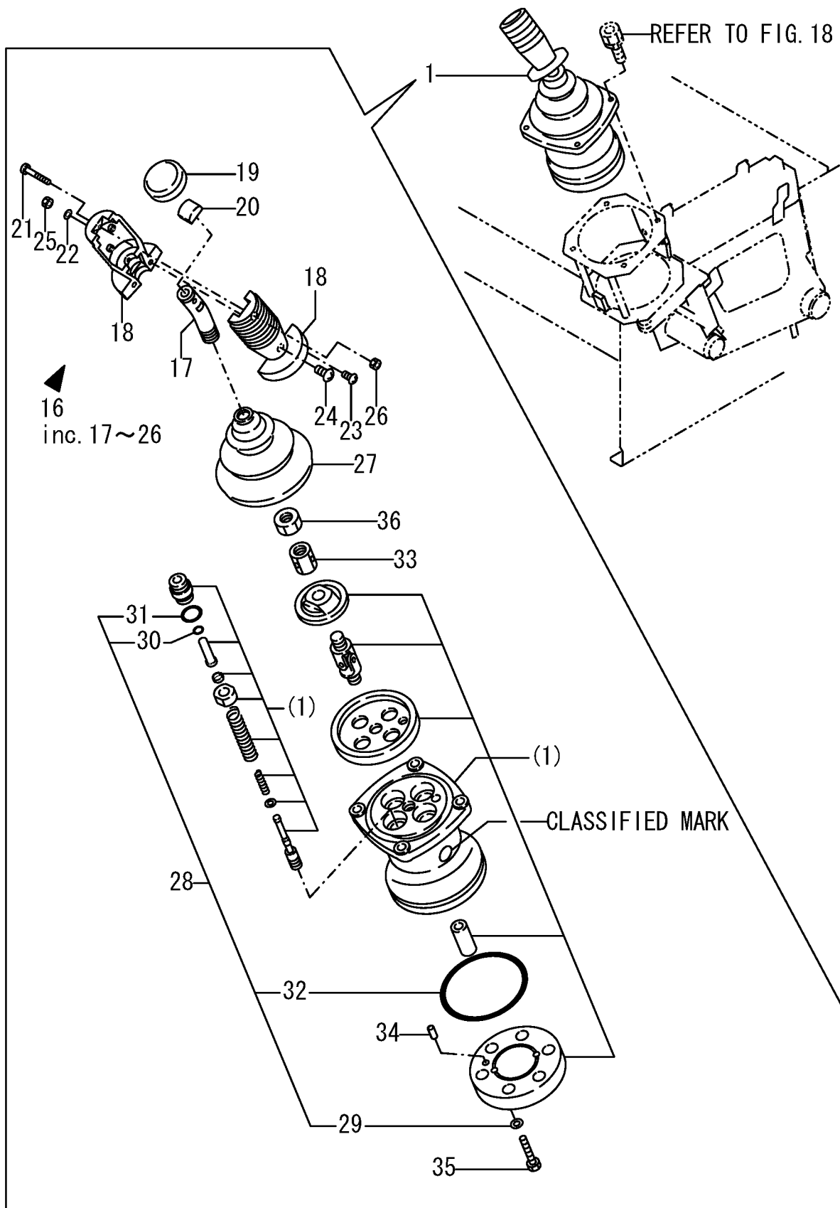
Fig. 49 REMOTE CONTROL VALVE (L)
