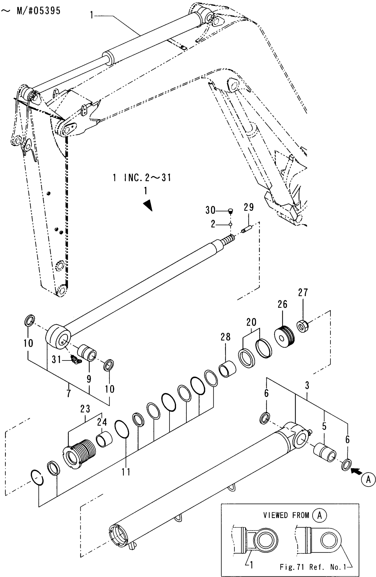
Fig. 40 ARM CYLINDER (PREVIOUS)
