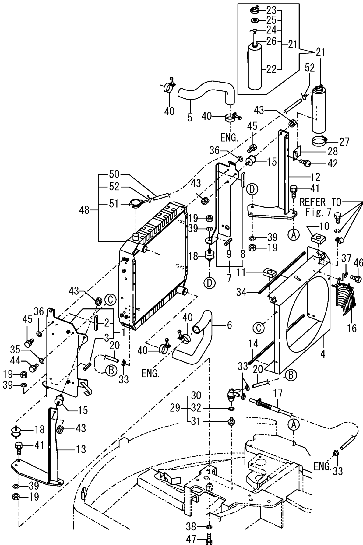
Fig. 6 RADIATOR & MOUNT
