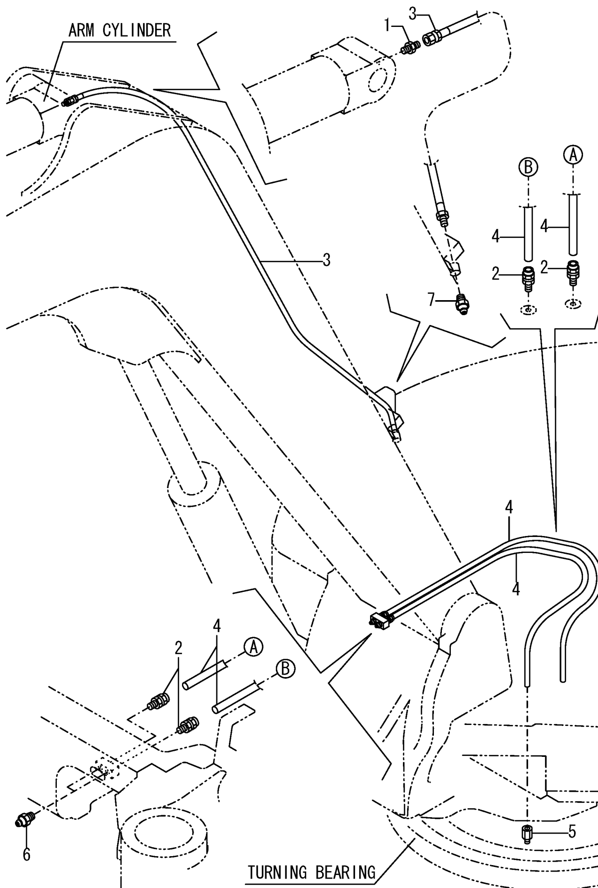
Fig. 64 GREASING
