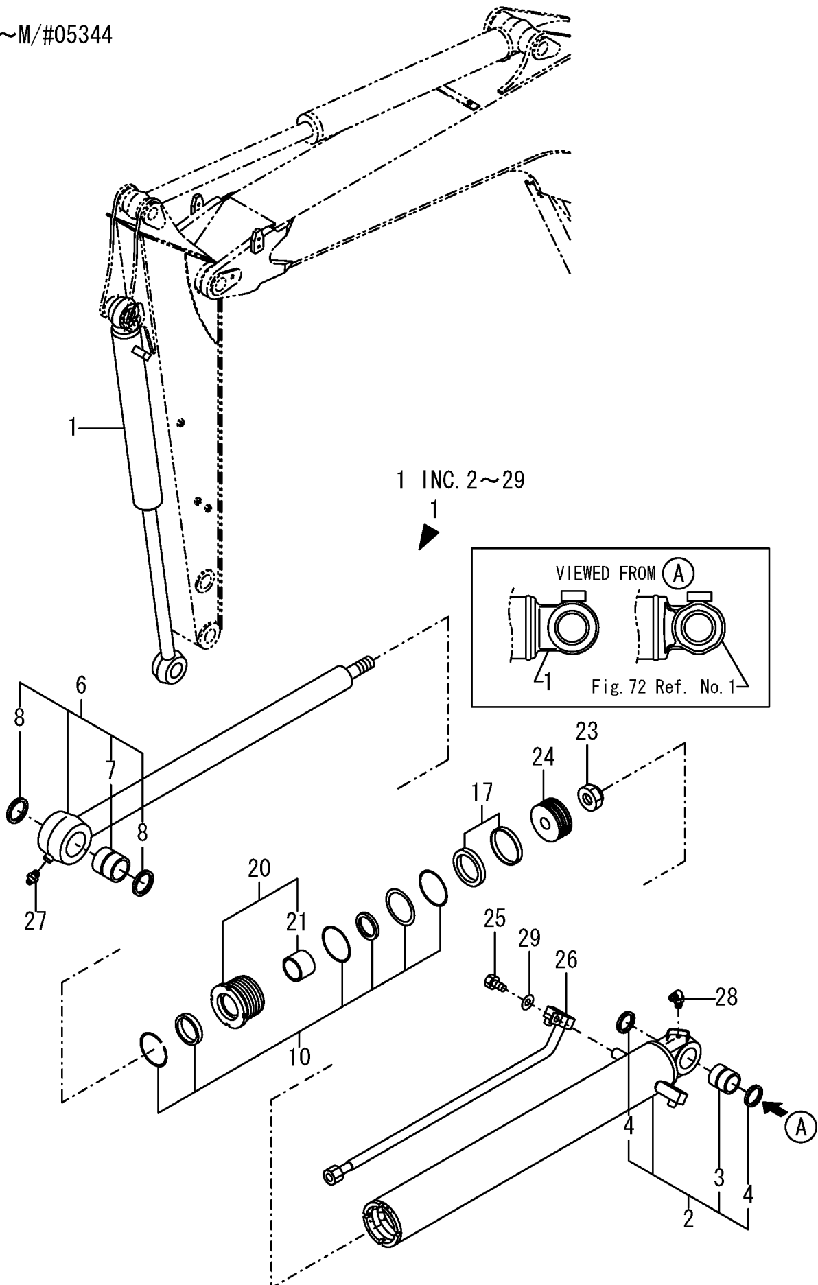
Fig. 41 BUCKET CYLINDER (PREVIOUS)
