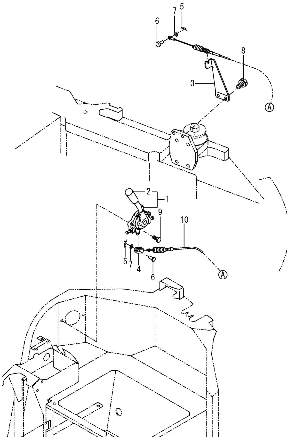
Fig. 4 ACCELERATOR
