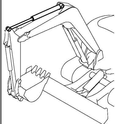
Fig. 40 ARM CYLINDER
