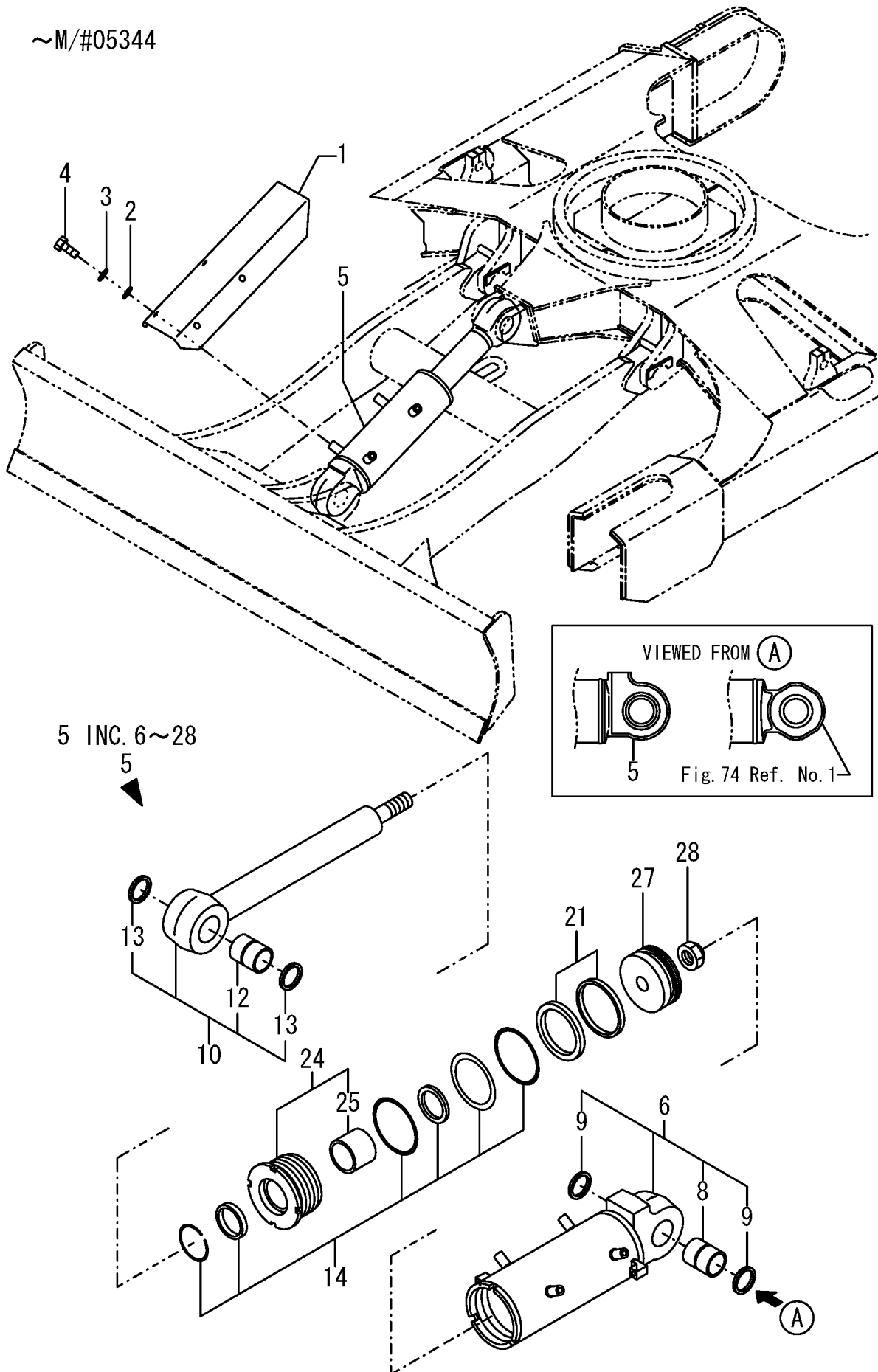
Fig. 43 BLADE CYLINDER (PREVIOUS)
