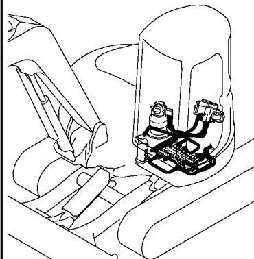
Fig. 58 HYD. OIL PIPING (P. T. O. FRAME END)
