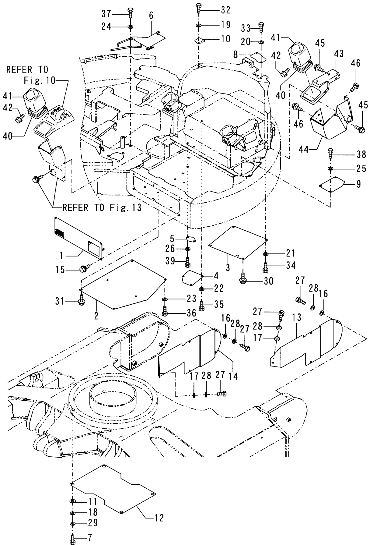
Fig. 25 FRAME COVER
