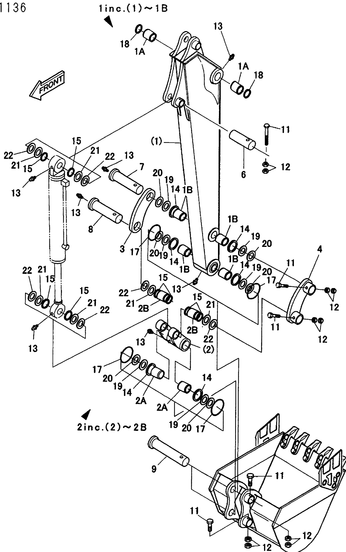
Fig. 132 ARM-1.6M (PREVIOUS)
