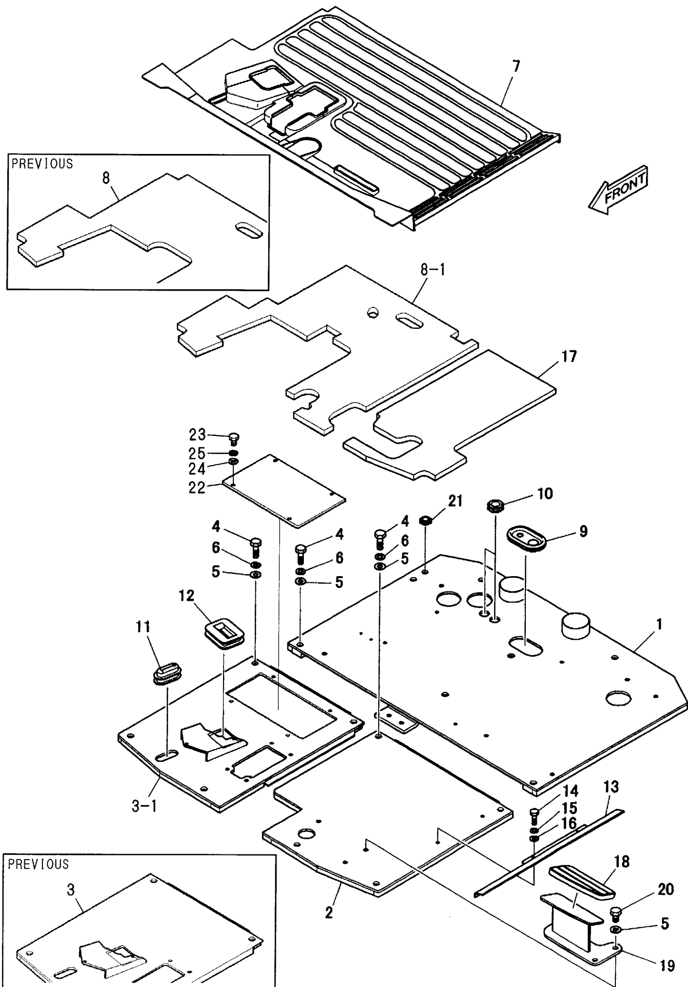
Fig. 38 FLOOR PLATE
