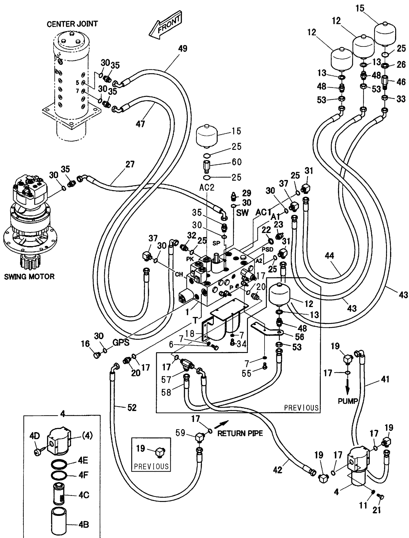
Fig. 119 BRAKE PIPING (2)
