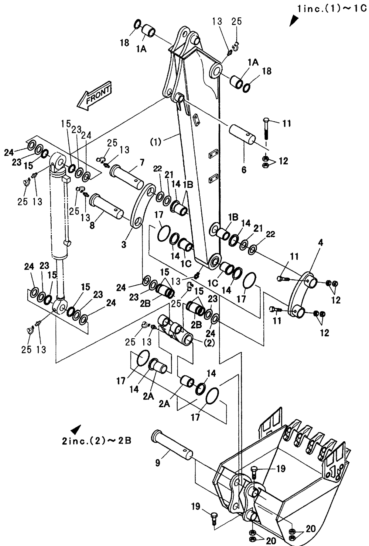
Fig. 59 ARM 1.6M-EXPORT
