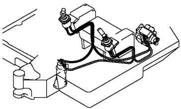
Fig. 49 CONTROL PIPING (PUMP ~ REMO.-CON. V. ~ RETURN)
