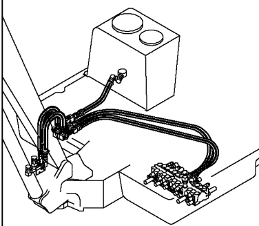
Fig. 46 HYD.OIL PIPING (TRAVEL)
