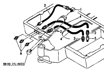
Fig. 51 GREASING
