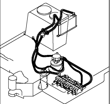
Fig. 44 HYD.OIL PIPING (RETURN:2)
