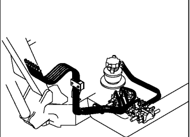
Fig. 41 HYD.OIL PIPING (VALVE ~ MOTOR, BOOM)
