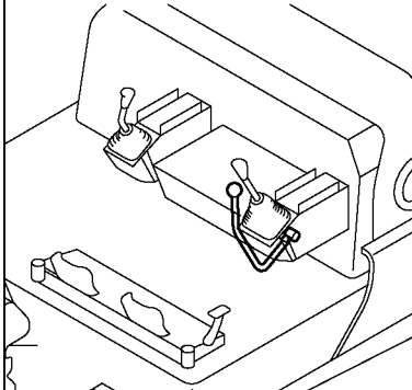
Fig. 18 CONTROL EQUIPMENT (P.T.O. CONTROL)
